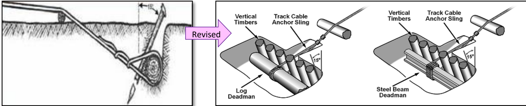
ATP 4-31, Recovery and Battle Damage Assessment and Repair: Log Deadman; before and after. Notice how the use of perspective brings out the engineering capability of its design function.
