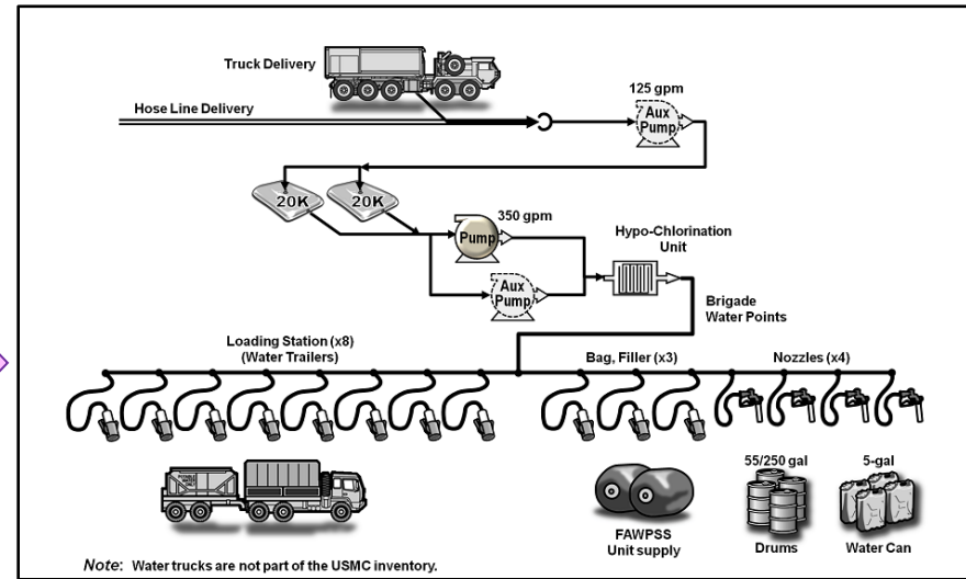
ATP 4-44: 40,000 Gallon water supply point setup; before and after. Notice the ability to create an embossed affect with PowerPoint.
