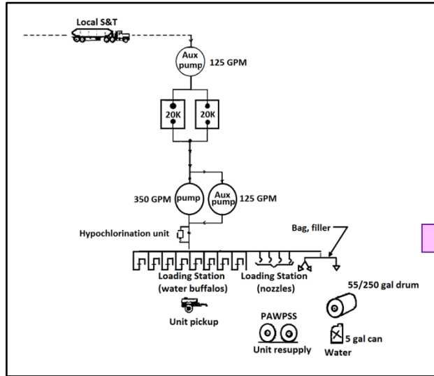
ATP 4-44: 40,000 Gallon water supply point setup; before and after. Notice the ability to create an embossed affect with PowerPoint.
