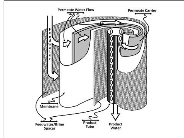
ATP 4-44, Water Supply in Theaters of Operations: Spiral RO Membrane Assembly; before and after.
