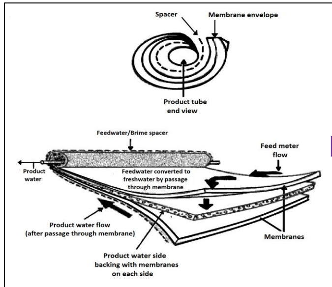
ATP 4-44, Water Supply in Theaters of Operations: Spiral RO Membrane Assembly; before and after.
