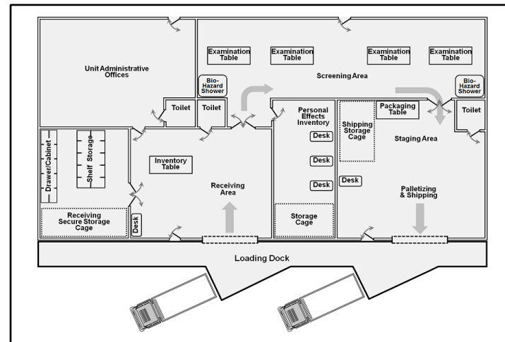
ATP 4-46, Mortuary Affairs Operations: Personal Affects Depot Layout, Visio versus PowerPoint
